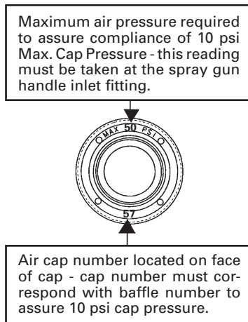
Figure 1 Baffle
